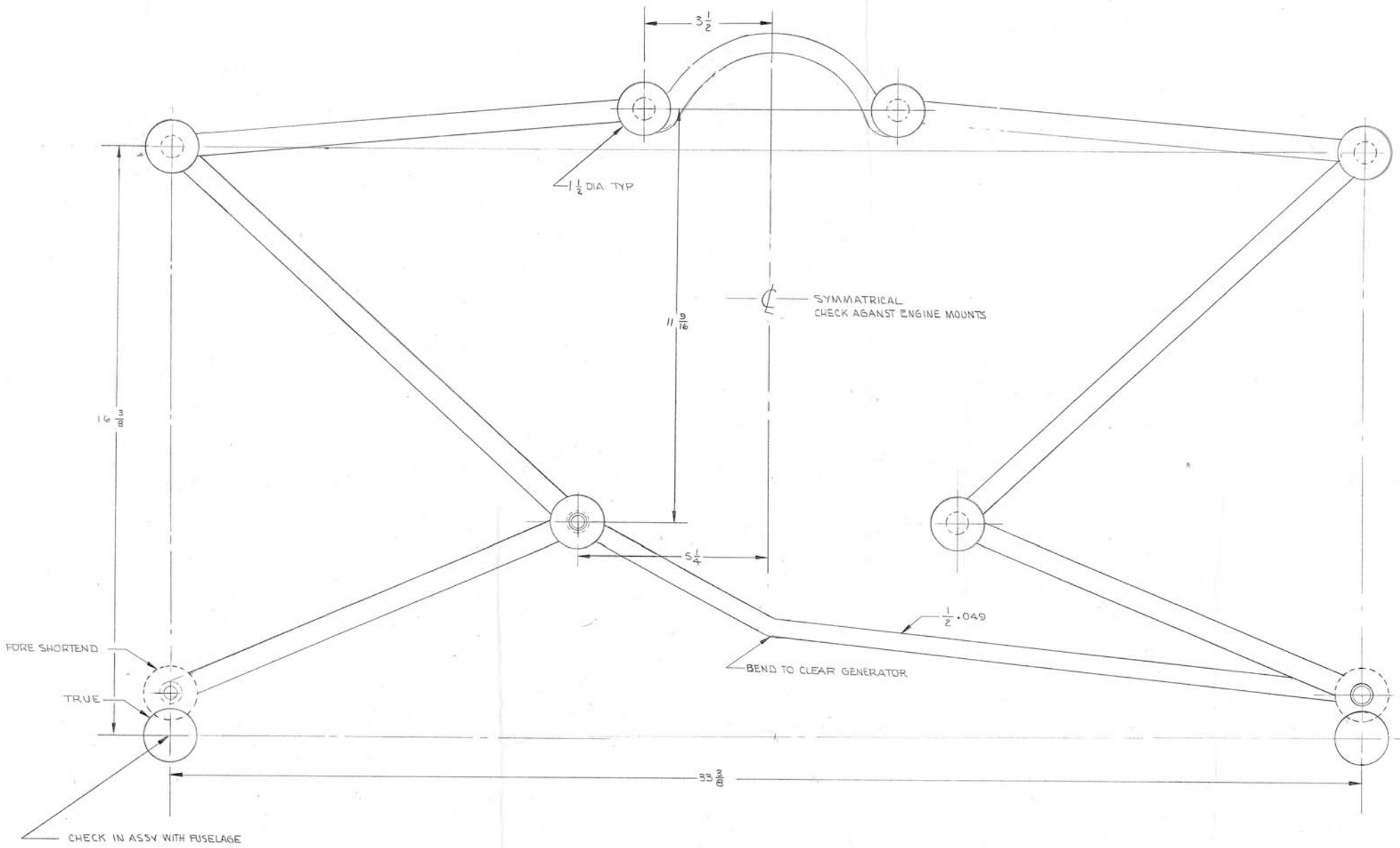
FRONT VIEW
